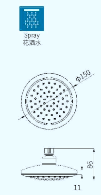
B25111 6" Rain shower 6寸圆形顶喷
