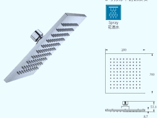
B30311 8"Stainless Steel Rain Shower Head 8 寸方形不锈钢顶喷
