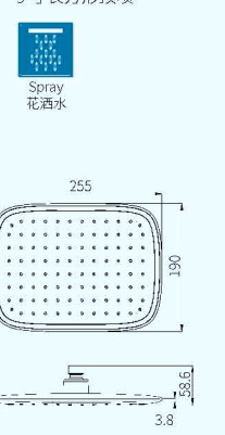
B28311 9" Rain shower 9寸长方形顶喷
