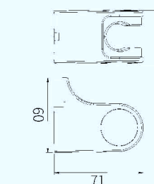
F42602 Adjustable wall bracket 免打孔可调式墙座
