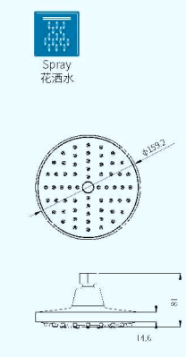
B25711 6" Rain shower 6寸圆形顶喷
