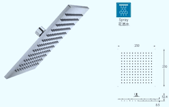
B30011 10"Stainless Steel Rain Shower Head 10 寸方形不锈钢顶喷
